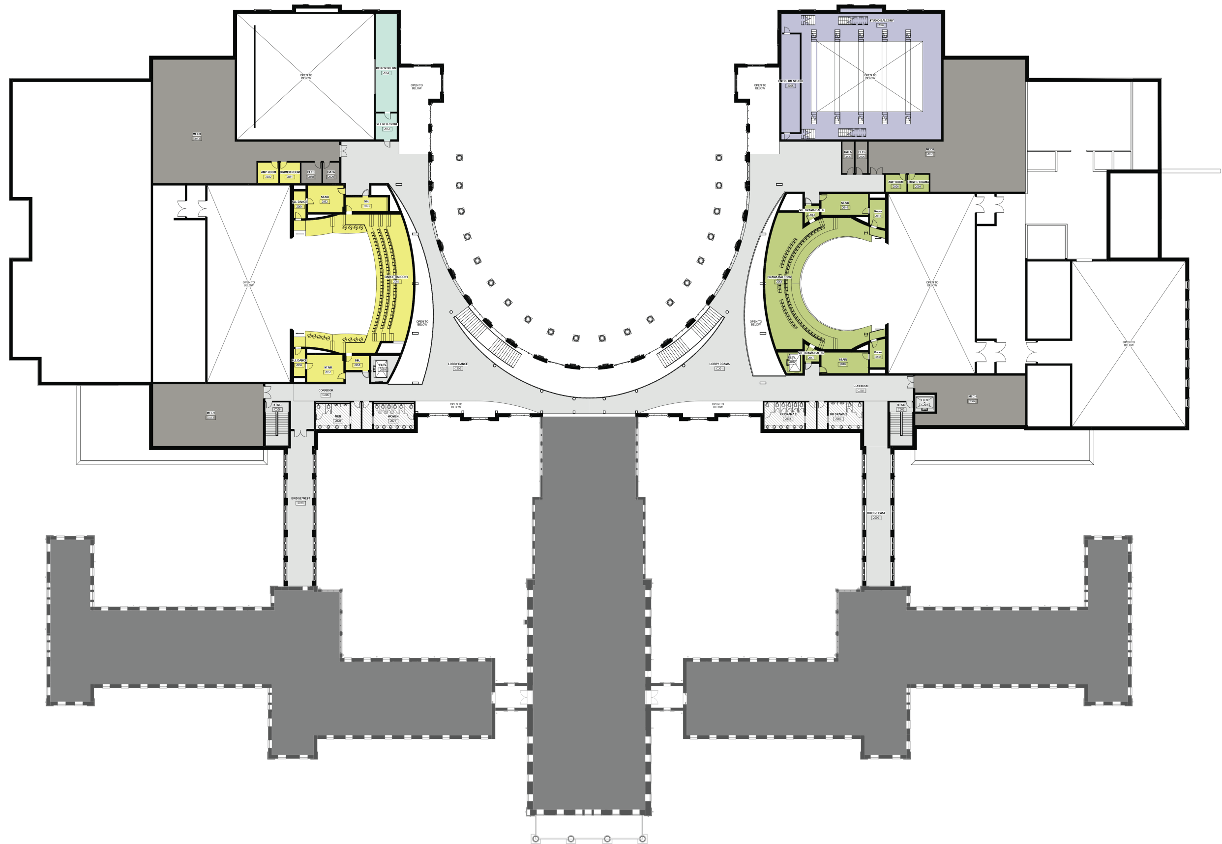
PERFORMING ARTS ACADEMIC CENTER | SECOND FLOOR
